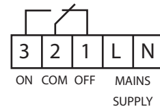
INTERNAL WIRING DIAGRAM CDTP2
