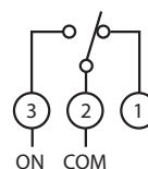
INTERNAL WIRING DIAGRAM CRTP2
